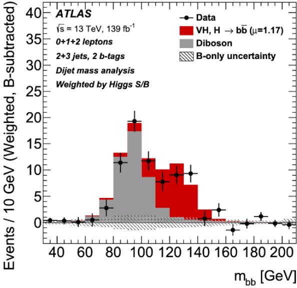
Fig. 15. The invariant mass distribution of a pair of b-jets obtained in pp collisions at an energy of 13 TeV in the ATLAS experiment in the processes of associated production of the Higgs boson with W and Z bosons and its decay into a pair of b-quarks. The contribution from all background processes is subtracted, with the exception of WZ and ZZ
