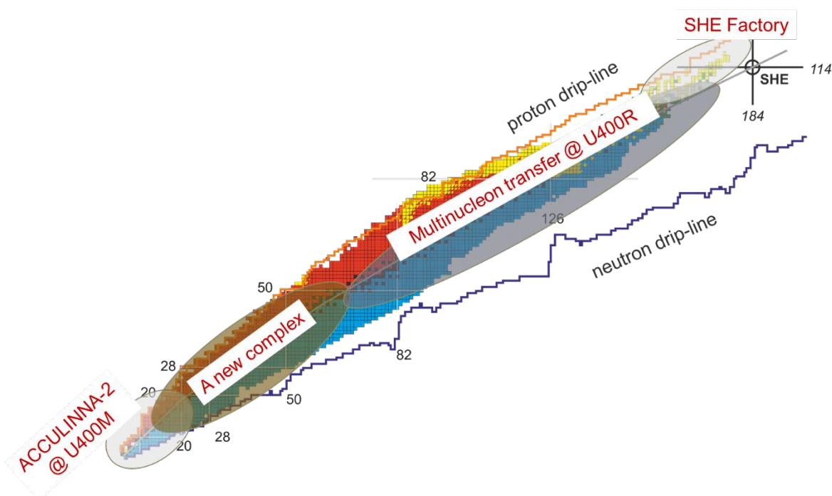
Fig. 21. Methods for obtaining nuclei in different areas of the nuclear map, developed at FLNR
