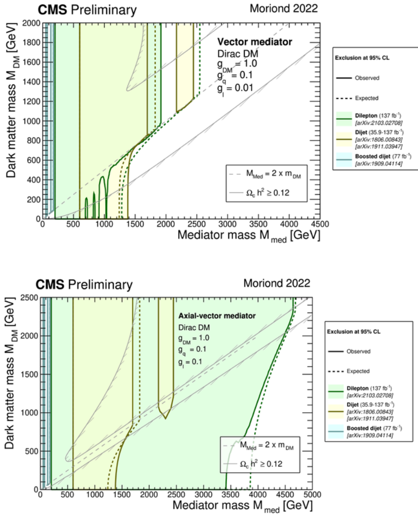
Fig. 16. In the combined channel of the production of a pair of jets and a pair of leptons in the events obtained in the CMS experiment at the LHC, the limits (95% C.L.) were determined on the masses of particle candidates for the role of dark matter particle m_{DM} and the mediator M_{med} . The shaded area corresponds to the excluded mass values for the vector (top) and pseudo-vector (bottom) mediator
