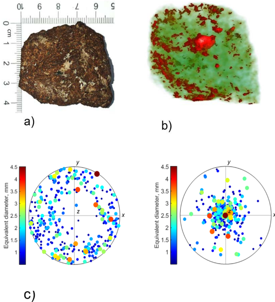
Fig. 30. Study of the internal structure and phase composition of a fragment of the Kunya-Urgench chondrite meteorite, known as the “Turkmenbashi meteorite”, which is one of the three largest known meteorites in the world. Photo (a) and a three-dimensional model (b) of a fragment of the Kunya-Urgench meteorite reconstructed from the neutron tomography data. Iron-nickel metallic components are marked in red. The pole figures of orientation of the main axes of inertia of the particles of FeNi kamacite of the Kunya-Urgench meteorite are also presented (c). The size of the symbols is proportional to the equivalent diameter of the metal particles
