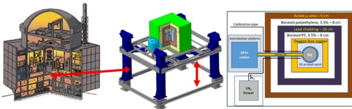
Fig. 19. Scheme of the vGeN setup aimed at detecting CEvNS. The setup is located directly under the KNPP reactor #3 (left), on a special lifting device (center) that allows changing the antineutrino flux in the HPGe detector, surrounded by a complex active and passive shielding (right)
