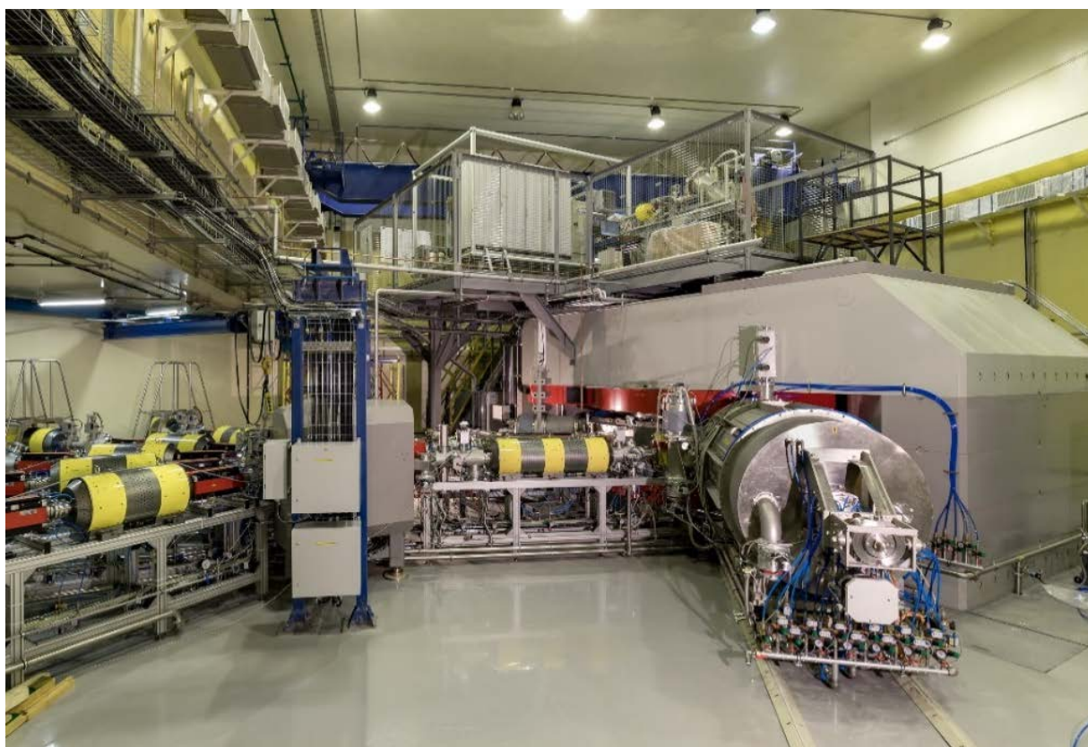
Fig. 20. DC-280 Cyclotron of the SHE Factory
