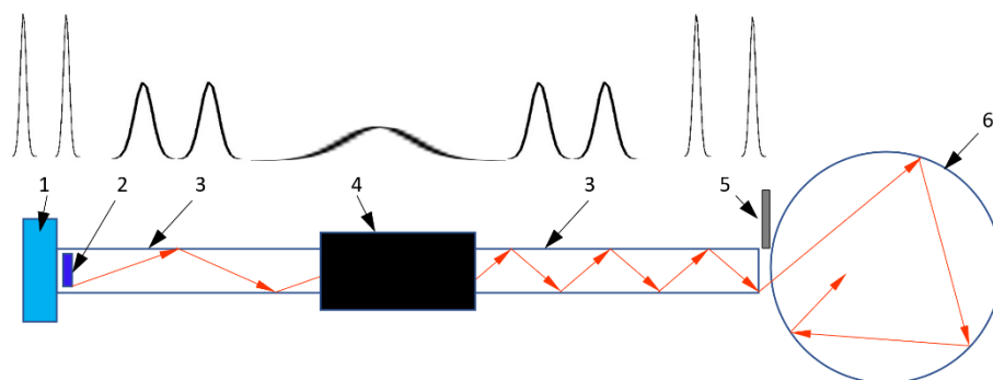
Fig. 25. The idea of an UCN source for a pulsed source using time focusing: 1 – moderator; 2 – UCN converter; 3 – mirror neutron guide; 4 – focusing device; 5 – fast shutter; 6 – UCN trap
