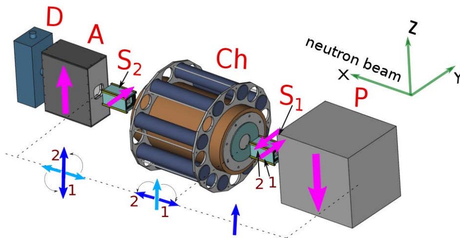
Fig. 23. Scheme of the experiment for measuring T-odd effects in fission. P – SEOP polarizer; Ch – fission chamber surrounded by gamma detectors; A – analyzer; D – neutron detector; S1, S2 – spin control devices. The pink arrows in the figure indicates the direction of the magnetic field, the blue arrows – the direction of the neutron spin
