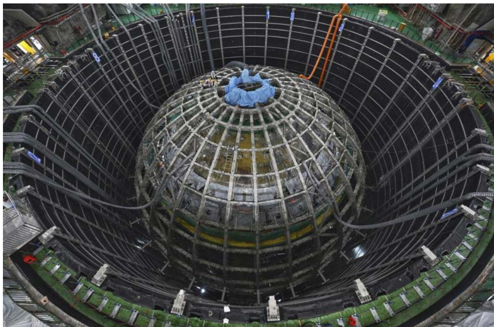
Fig. 17. Current status of the JUNO detector assembly
