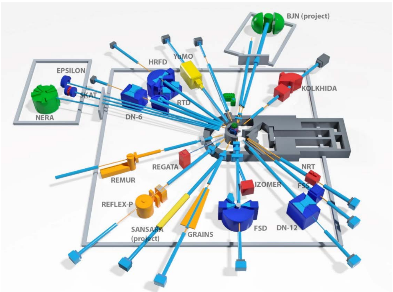
Fig. 7. IBR-2 spectrometer complex
